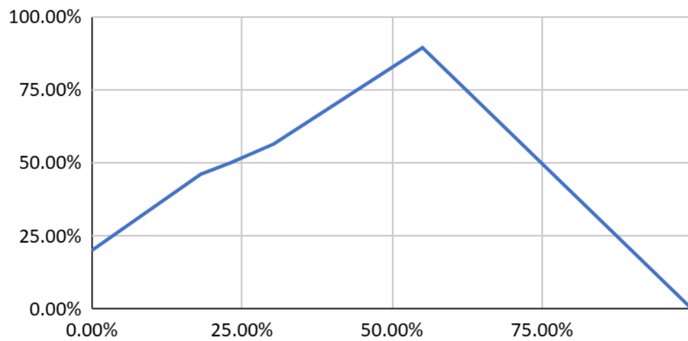
FPR (Error Type 2) and Sensitivity
