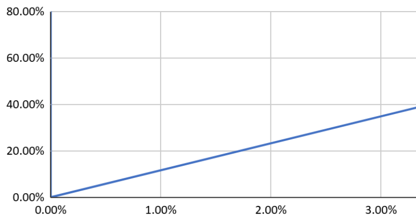
FPR (Error Type 2) and Sensitivity
