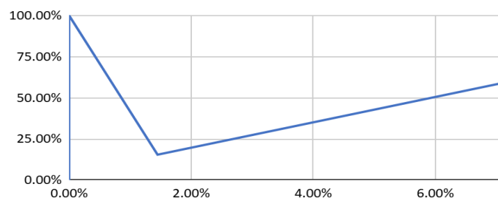
FPR (Error Type 2) and Sensitivity
