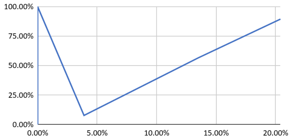
FPR (Error Type 2) and Sensitivity
