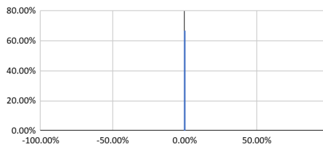
FPR (Error Type 2) and Sensitivity
